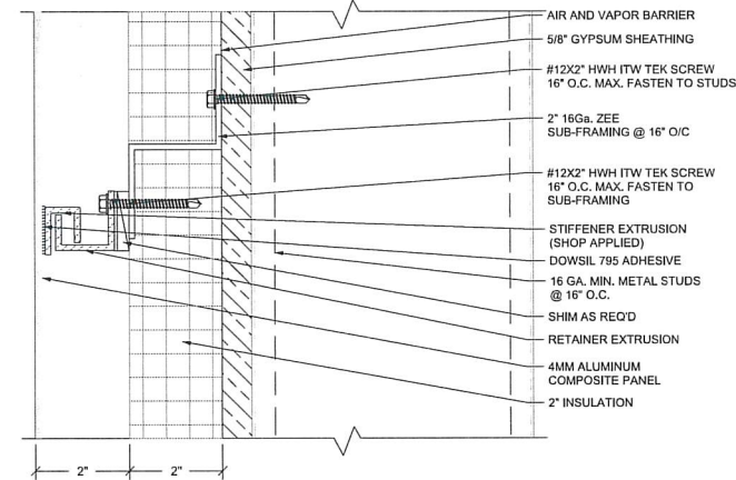
6 3.2 STIFFENER/RETAINER DETAIL REF: NONE SCALE: 6"=1'-0"
