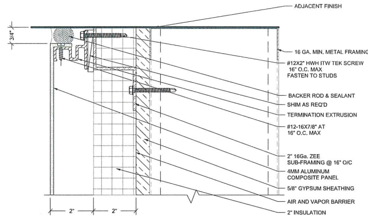
1 3.3 HEAD TERMINATION REF: NONE SCALE: 6"=1'-0"
