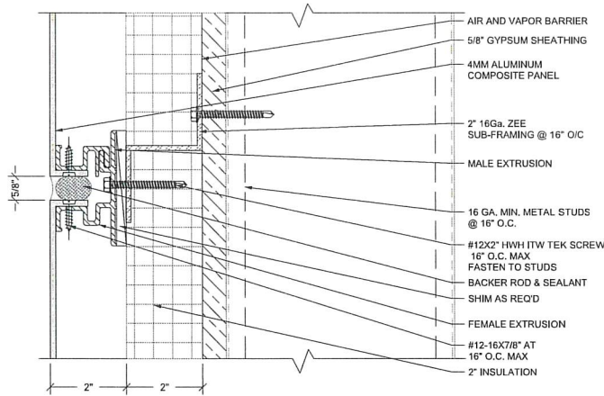
2 3.3 TYP. HORIZONTAL JOINT REF: NONE SCALE: 6"=1'-0"
