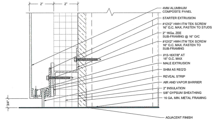
3 3.2 TYP. BASE TERMINATION REF: NONE SCALE: 6"=1'-0"
