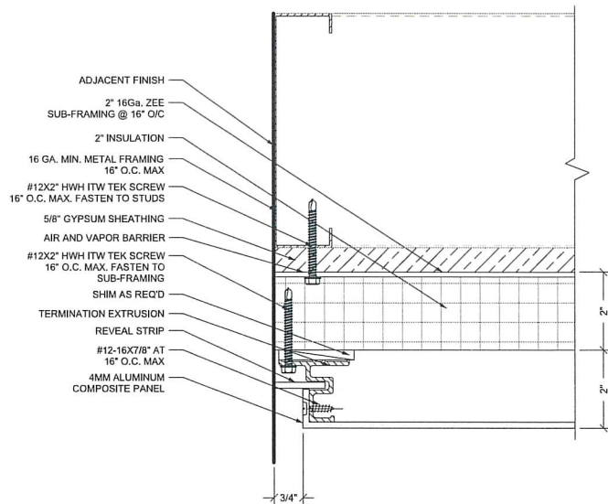
4 3.2 JAMB TERMINATION REF: NONE SCALE: 6"=1'-0"
