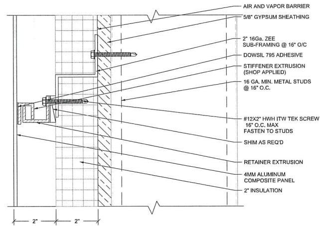
6 3.3 STIFFENER/RETAINER DETAIL REF: NONE SCALE: 6"=1'-0"
