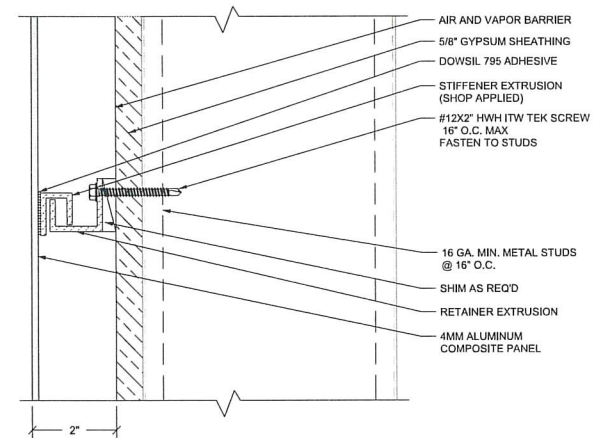
6 STIFFENER/RETAINER DETAIL 3.1 REF: NONE SCALE: 6"=1'-0"
