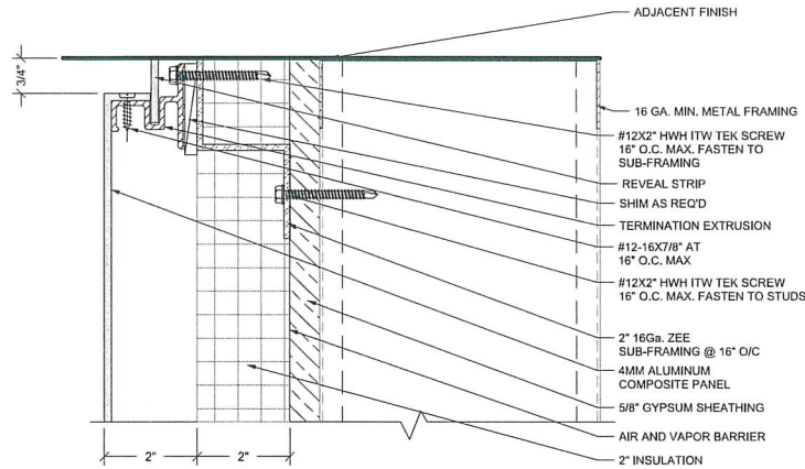
1 3.2 HEAD TERMINATION REF: NONE SCALE: 6"=1'-0"
