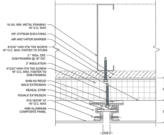
5 3.2 TYP. VERTICAL JOINT REF: NONE SCALE: 6"=1'-0"
