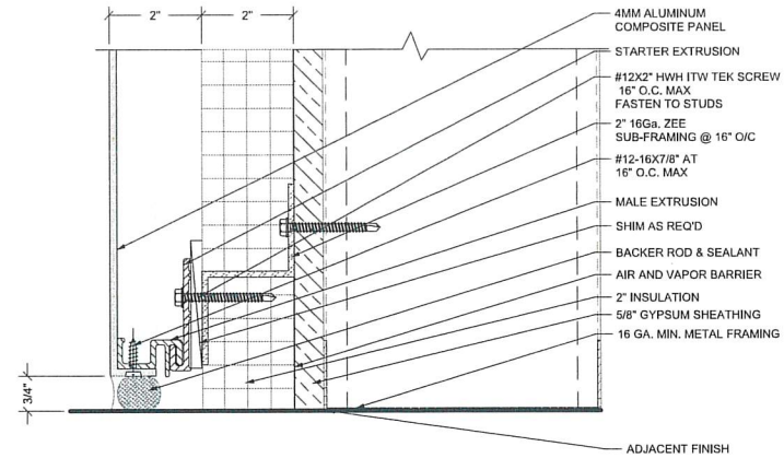
3 3.3 TYP. BASE TERMINATION REF: NONE SCALE: 6"=1'-0"
