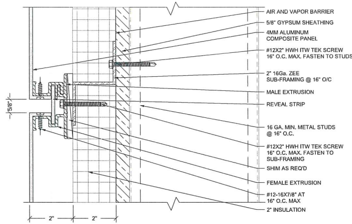
2 3.2 TYP. HORIZONTAL JOINT REF: NONE SCALE: 6"=1'-0"
